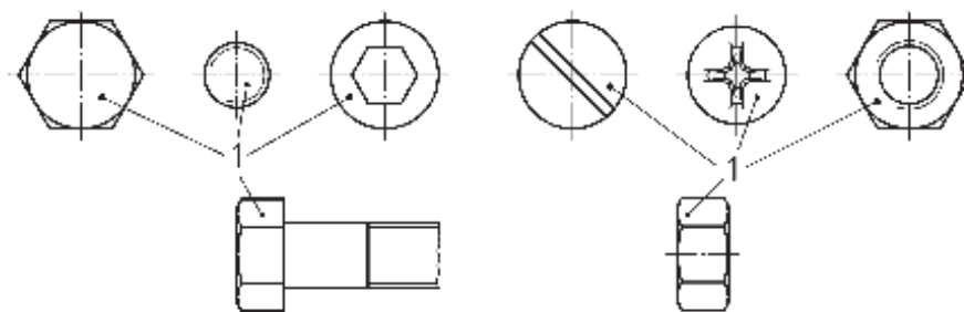
a) Reference areas for threaded fasteners
