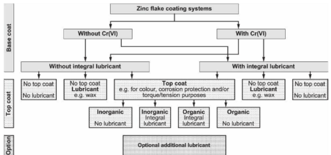
Figure A.1 — Typical zinc flake coating systems
