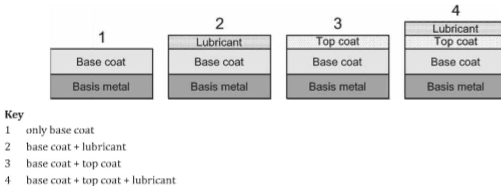
Figure 1 — Basic zinc flake coating systems
