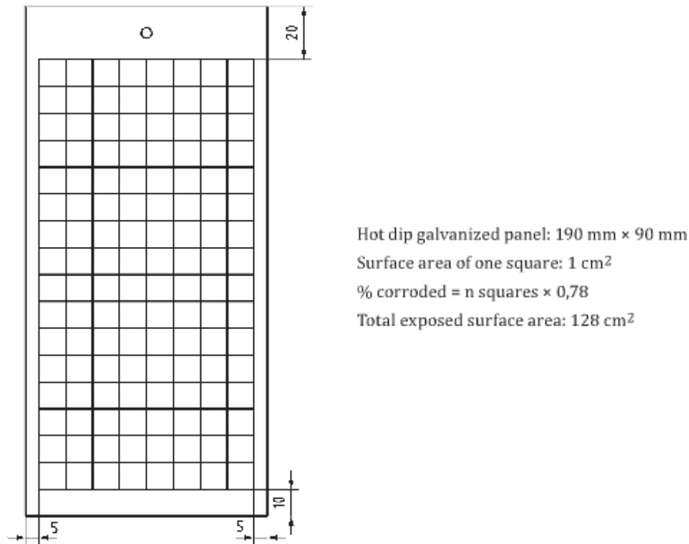
Figure C.4 — Protection and control mask for reference panels
