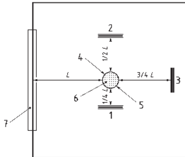
Figure C.2 — Centred spray cabinet
